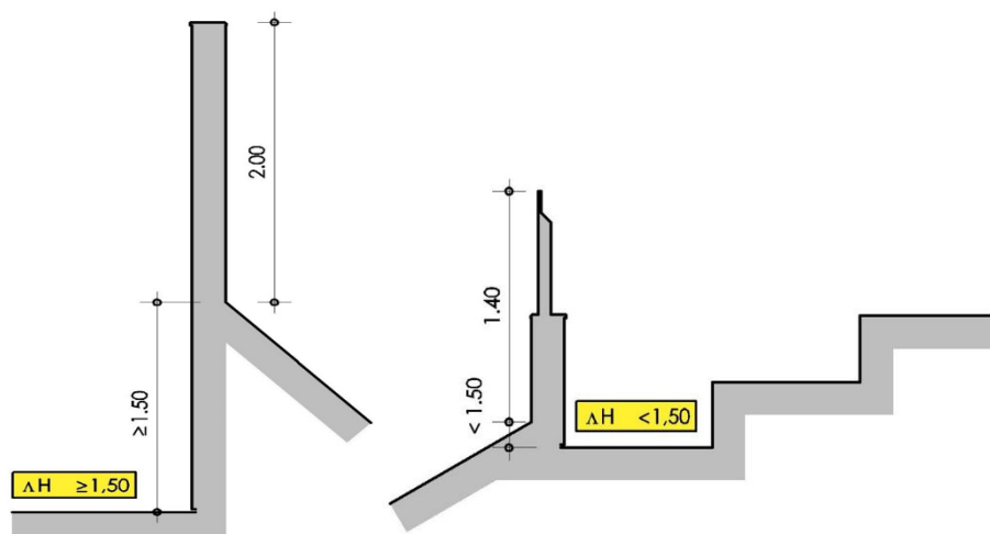
Diagram showing the outer fence at different heights
